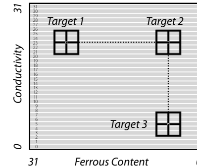
Targets 1 and 2 will produce an identical high tone response as their conductivity is the same (COND 23).
