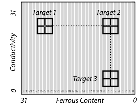
Targets 2 and 3 will produce an identical high tone response as their ferrous content is the same (FER 6).
