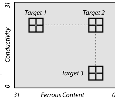
Targets 1, 2 and 3 will produce identical tone response.
